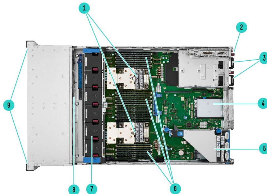
Internal View SFF chassis– Air Cooled
